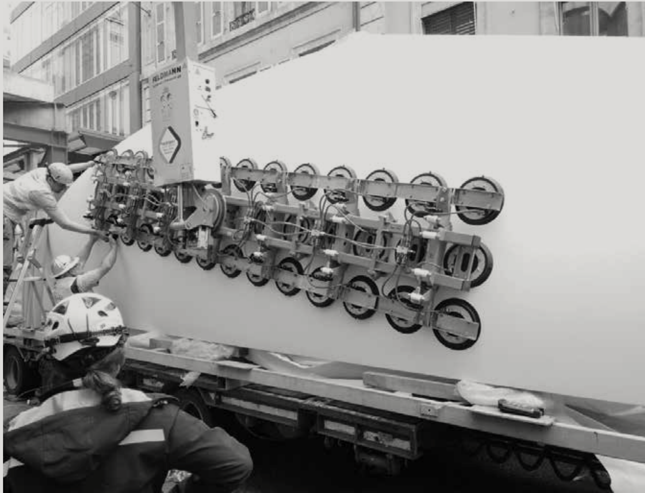
Transport, unloading, and handling phases of the GFRP modules
